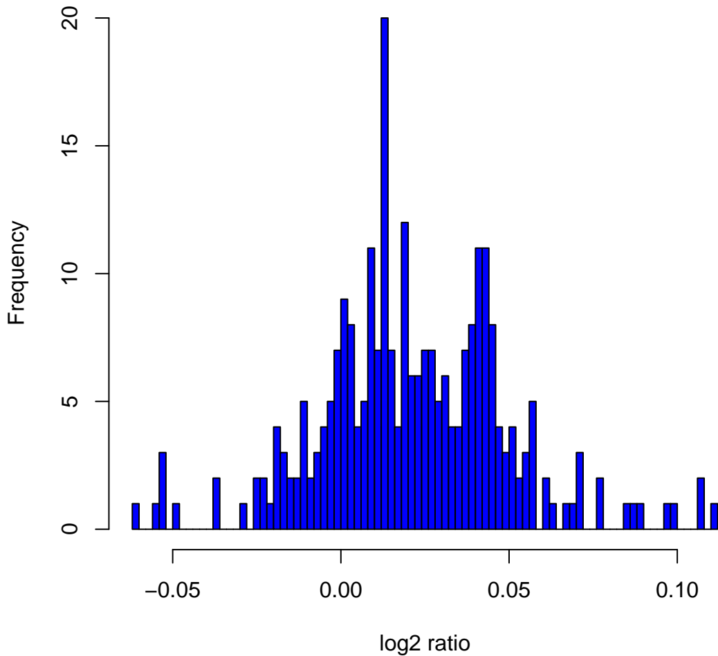
Histogram of log 2 ratios in 270 HapMap samples at clone Chr3tp-8C2
