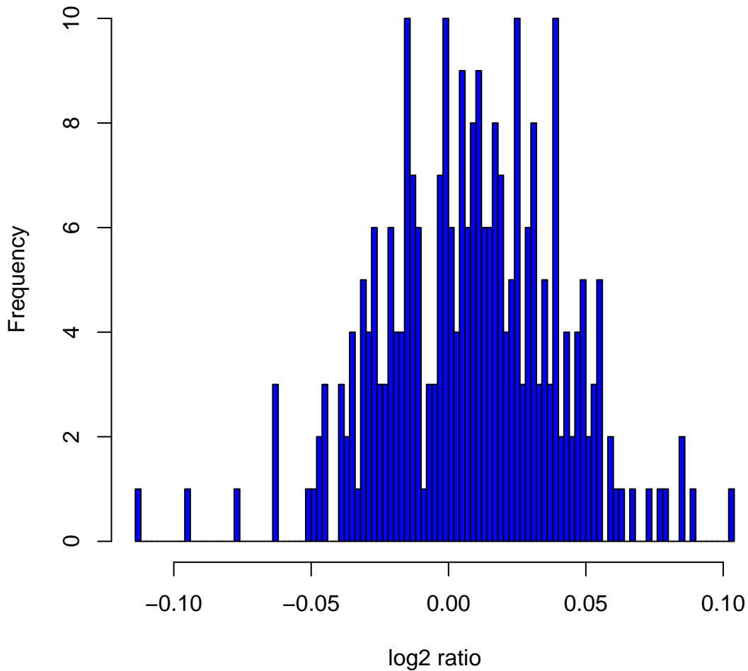
Histogram of log 2 ratios in 270 HapMap samples at clone Chr3tp-8C7
