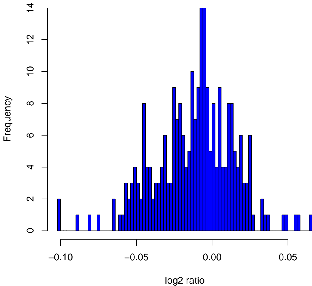
Histogram of log 2 ratios in 270 HapMap samples at clone Chr3tp-8D3
