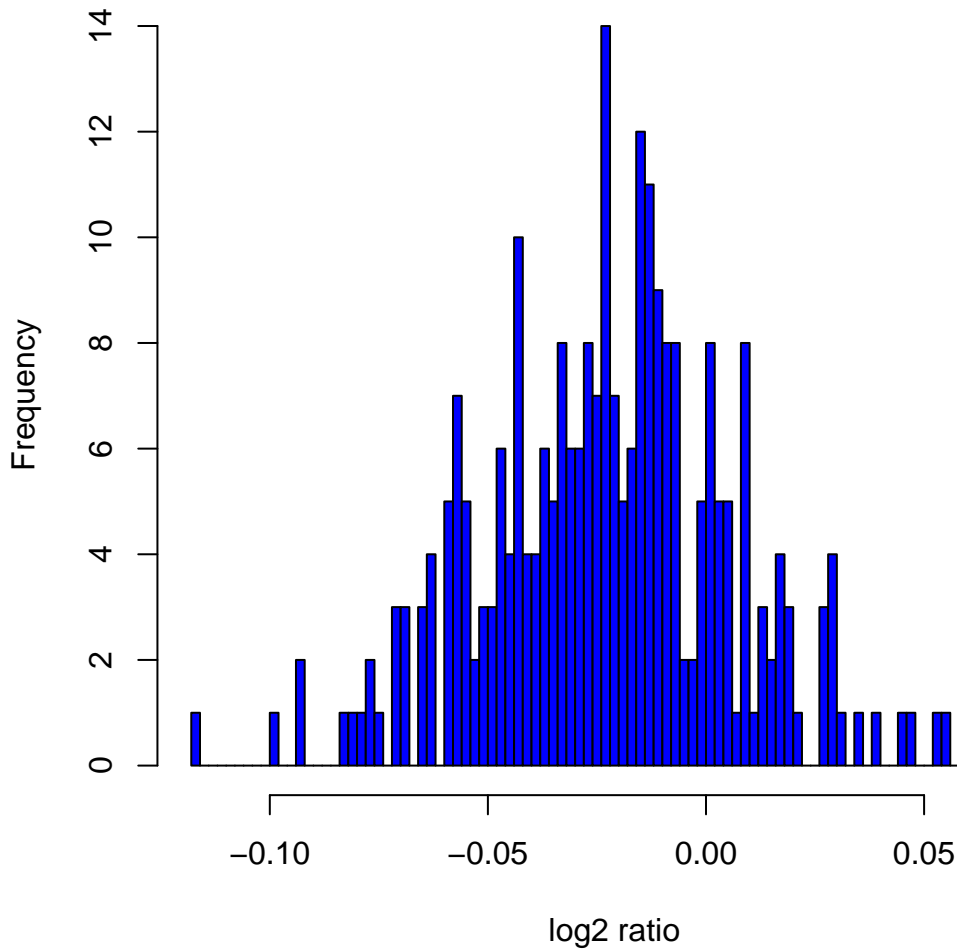
Histogram of log 2 ratios in 270 HapMap samples at clone Chr3tp-8E6
