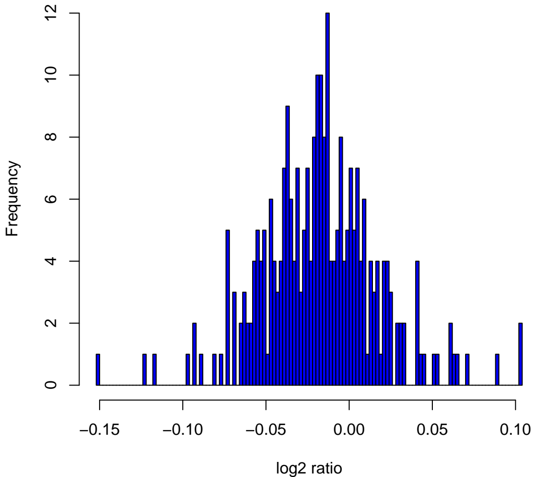
Histogram of log 2 ratios in 270 HapMap samples at clone Chr3tp-8E9
