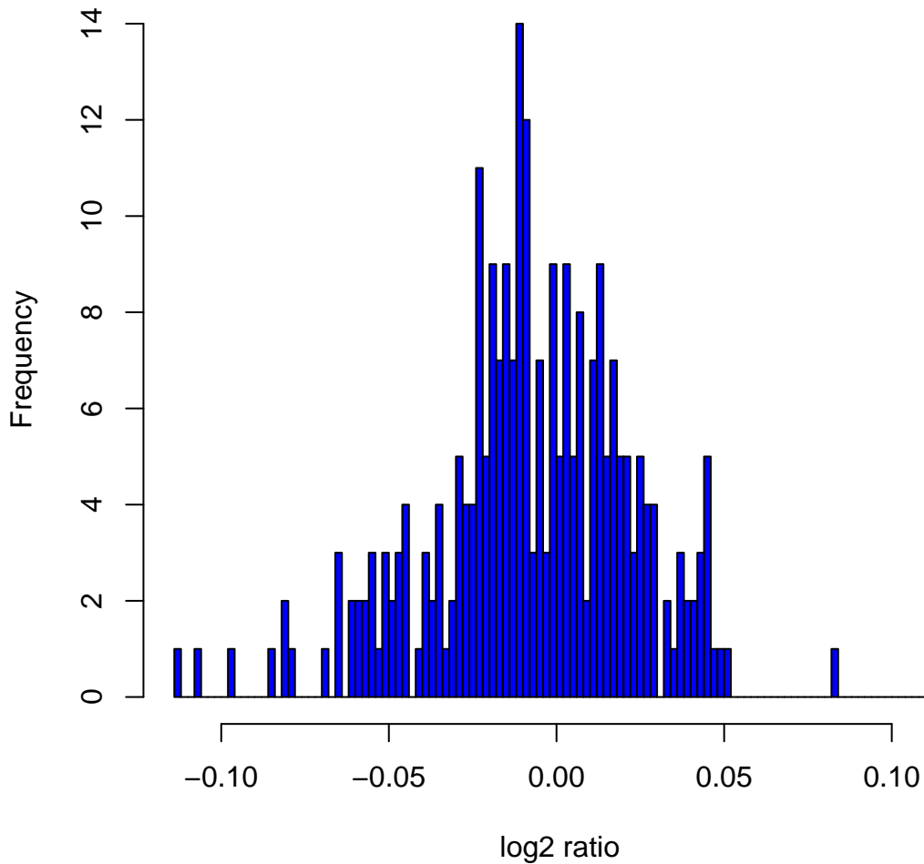
Histogram of log 2 ratios in 270 HapMap samples at clone Chr3tp-8G6
