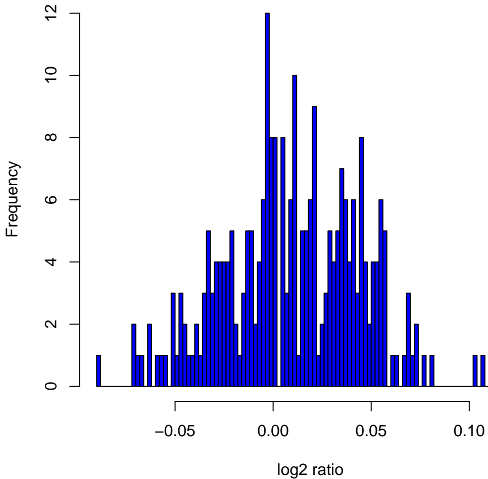
Histogram of log 2 ratios in 270 HapMap samples at clone Chr3tp-8H5
