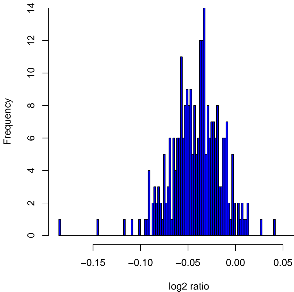
Histogram of log 2 ratios in 270 HapMap samples at clone Chr3tp-9A7
