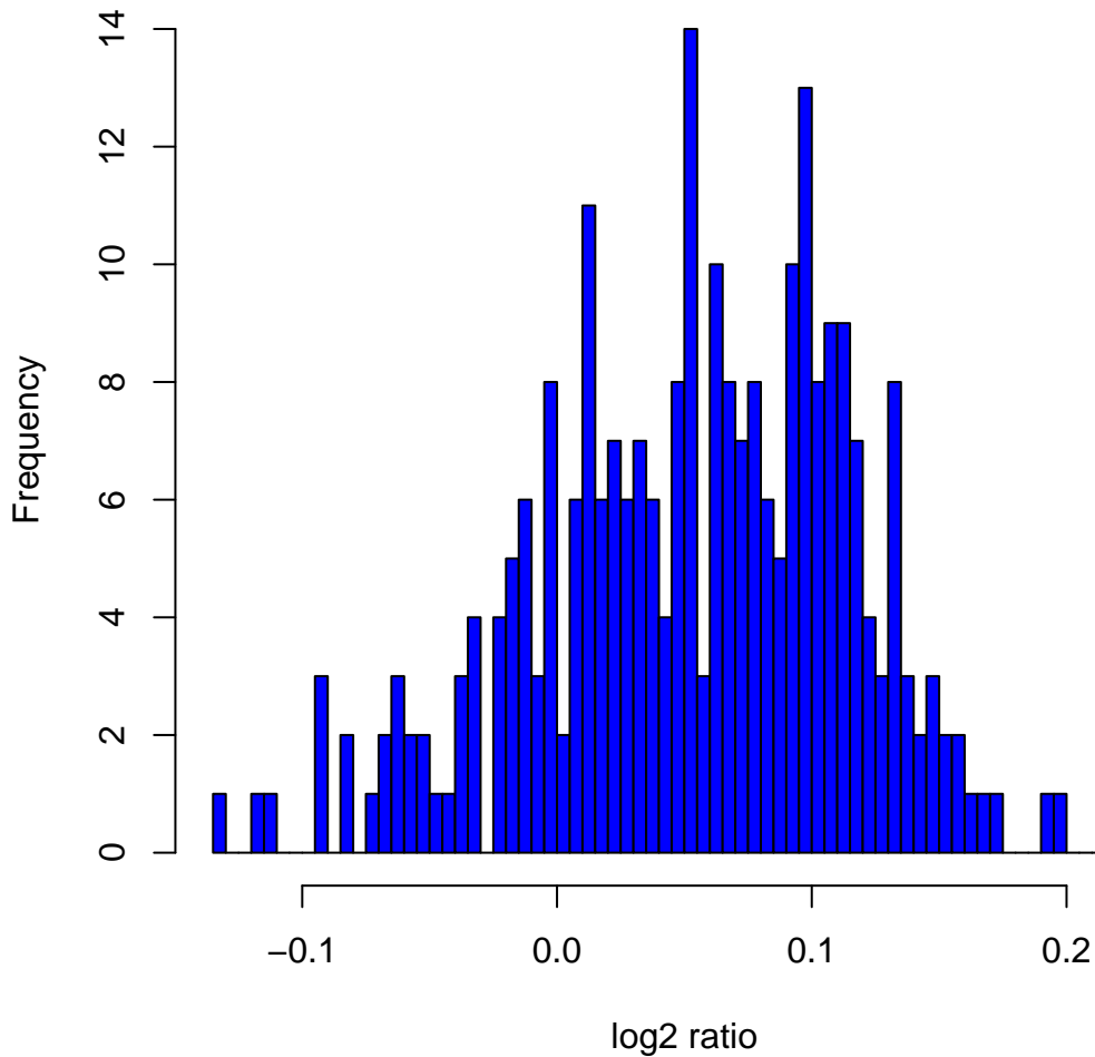
Histogram of \log_2 ratios in 270 HapMap samples at clone Chr3tp-9C3
