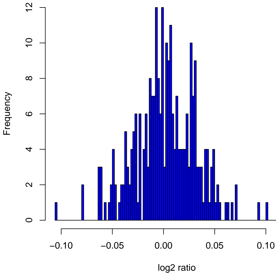
Histogram of log 2 ratios in 270 HapMap samples at clone Chr3tp-9E1
