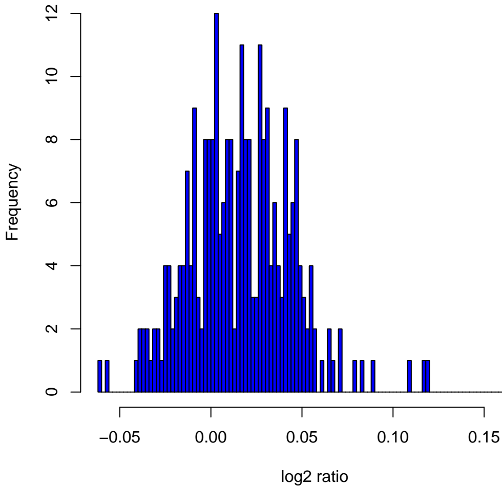
Histogram of log2ratios in 270 HapMap samples at clone Chr3tp-9E8
