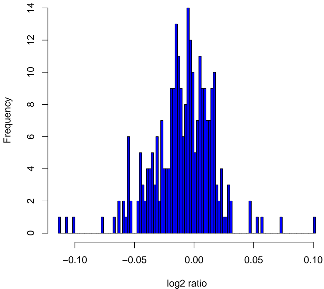
Histogram of \log_2 ratios in 270 HapMap samples at clone Chr3tp-9G5
