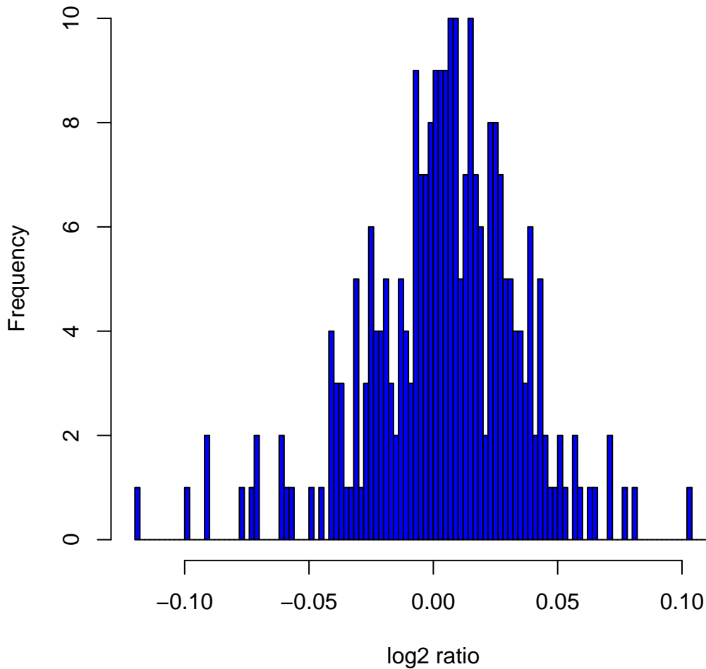
Histogram of log 2 ratios in 270 HapMap samples at clone Chr3tp-9H1
