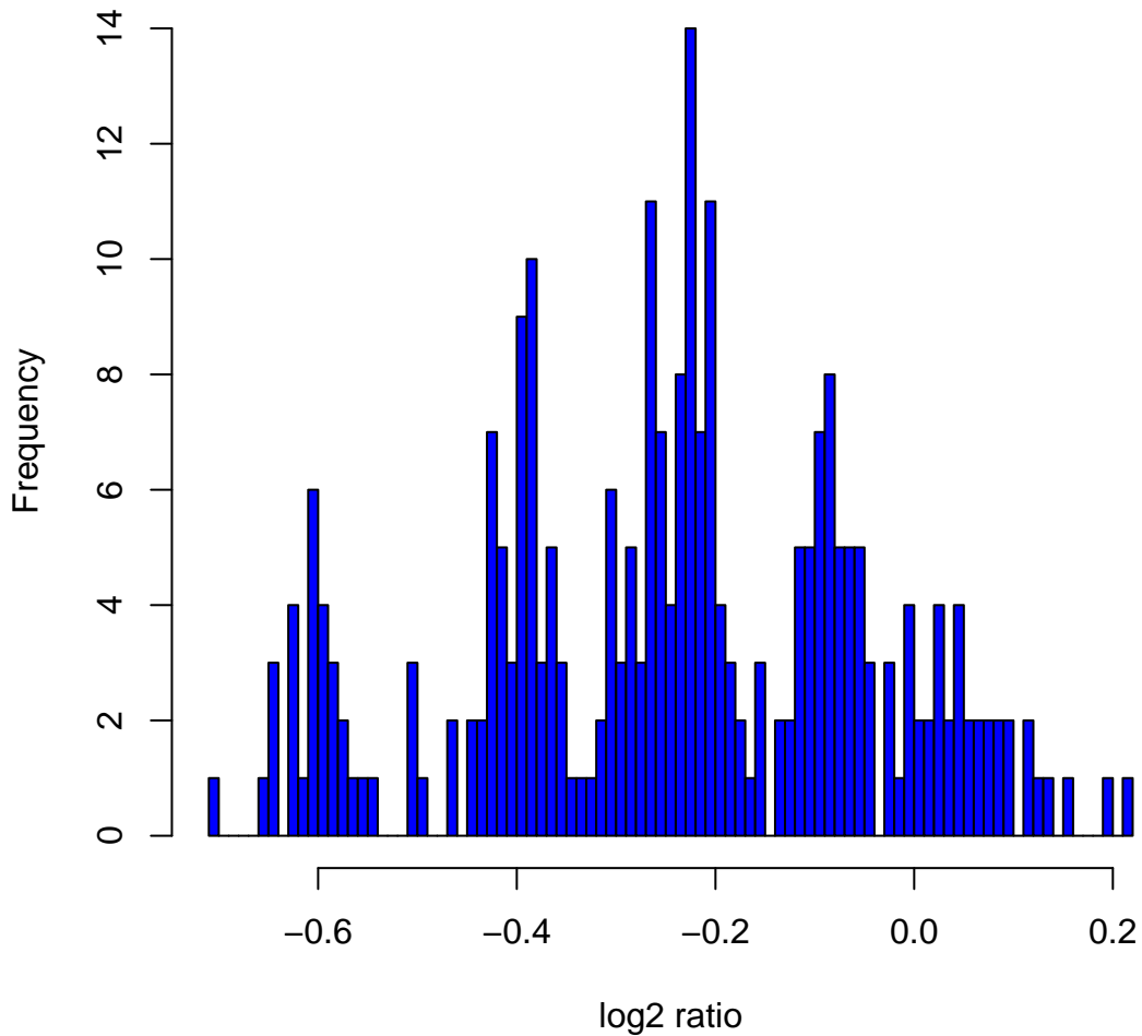
Histogram of \log_2 ratios in 270 HapMap samples at clone Chr3tp-9H6
