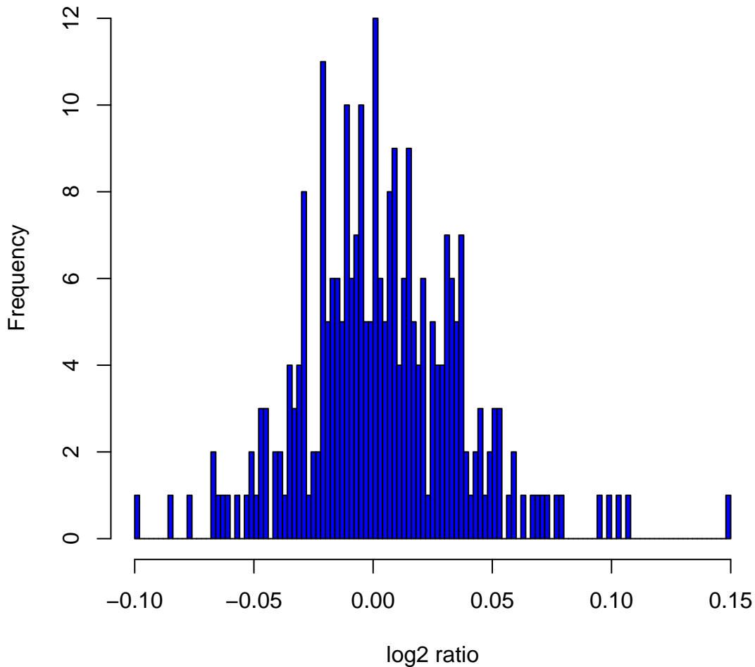
Histogram of \log_2 ratios in 270 HapMap samples at clone Chr3tp-9H7
