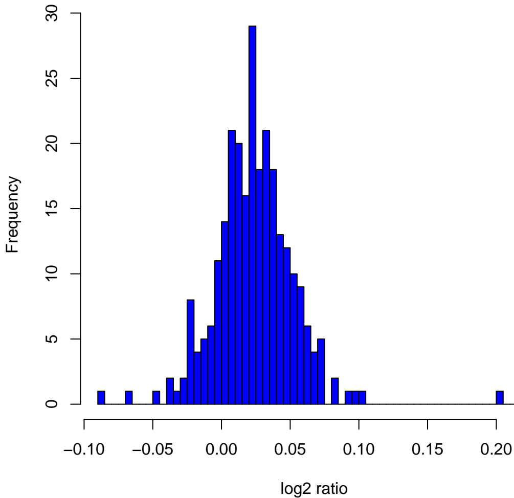
Histogram of \log_2 ratios in 270 HapMap samples at clone Chr8tp-7B11
