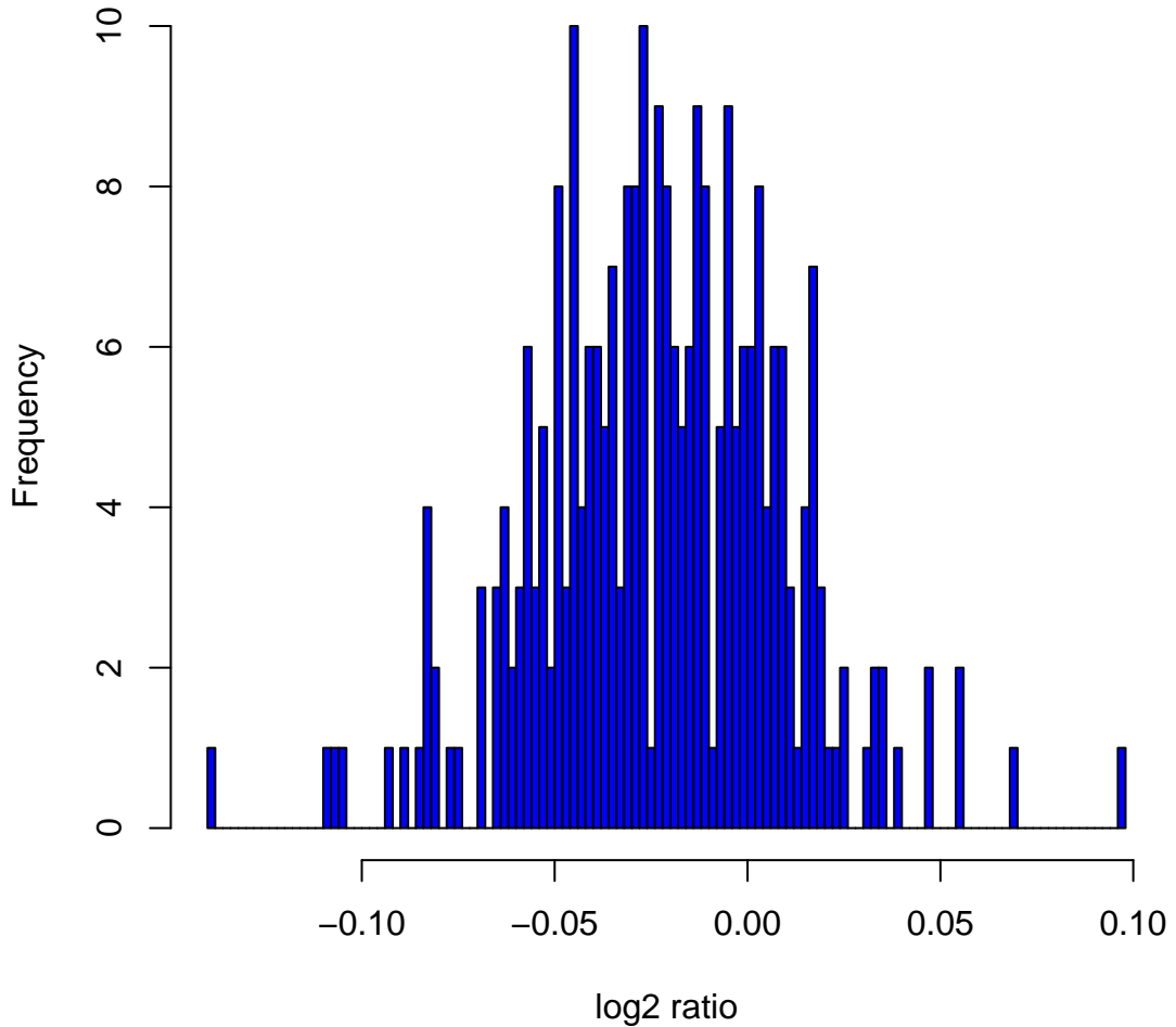
Histogram of log2ratios in 270 HapMap samples at clone Chr4tp-10H11
