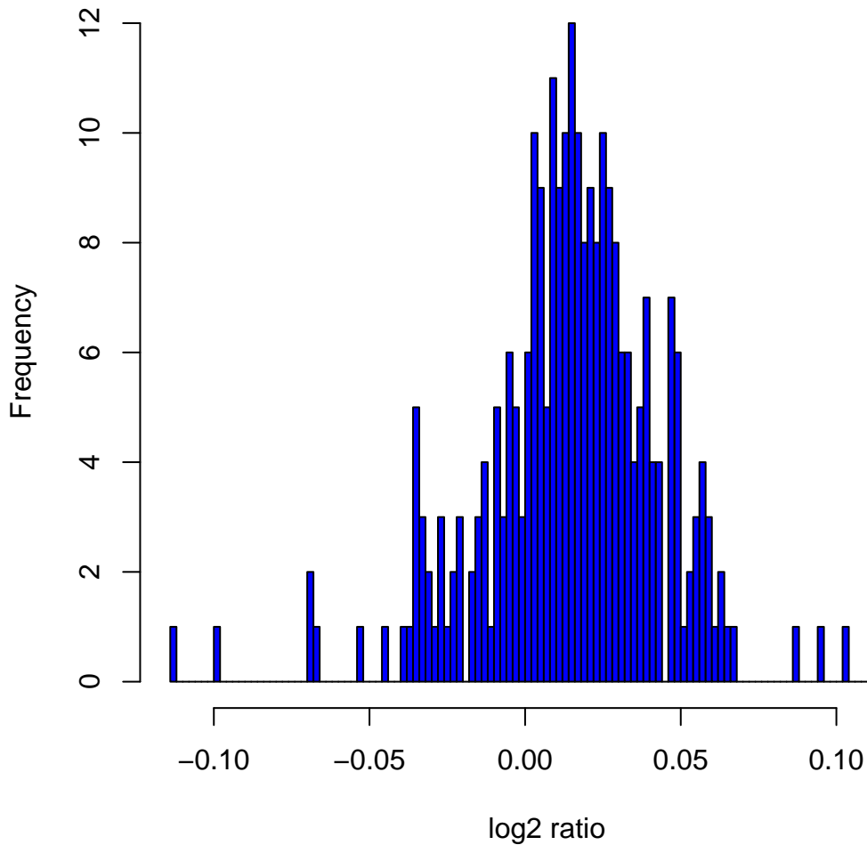
Histogram of log 2 ratios in 270 HapMap samples at clone Chr4tp-11B1
