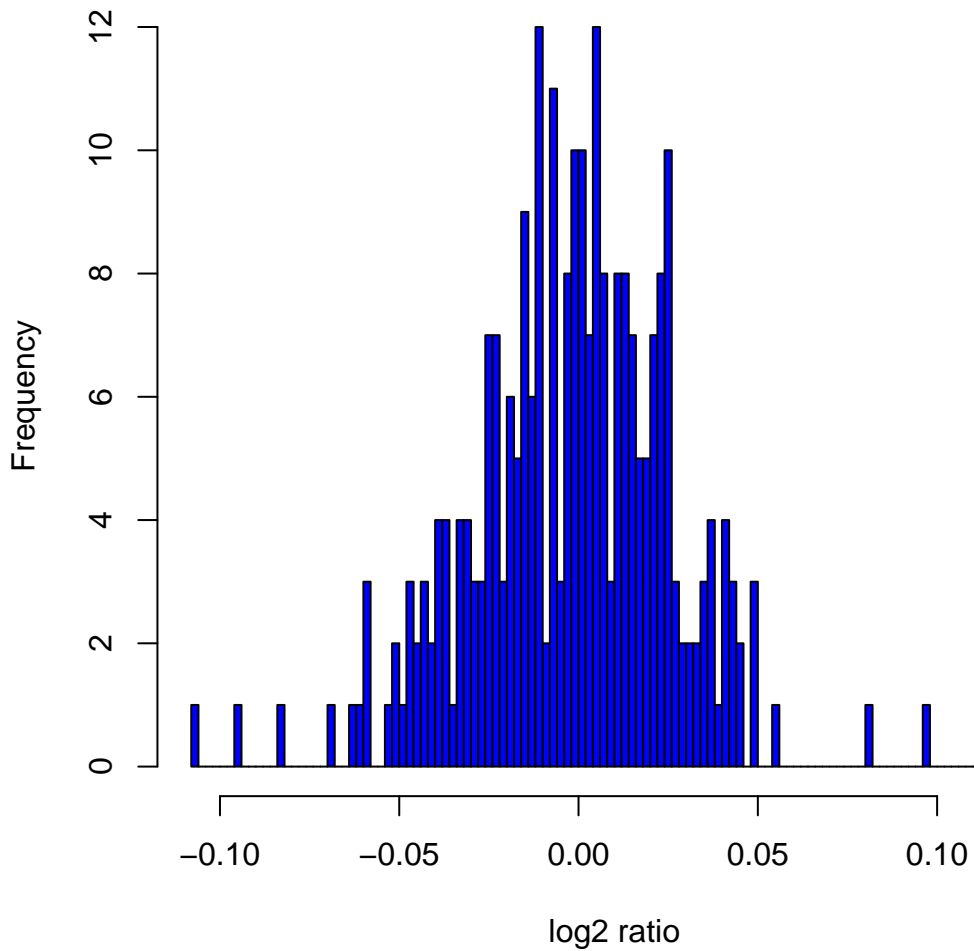
Histogram of log 2 ratios in 270 HapMap samples at clone Chr4tp-11B3
