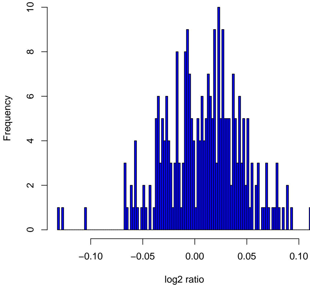
Histogram of log2ratios in 270 HapMap samples at clone Chr4tp-11C11
