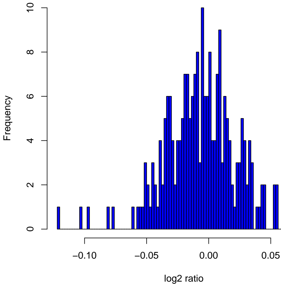
Histogram of log 2 ratios in 270 HapMap samples at clone Chr4tp-11F9
