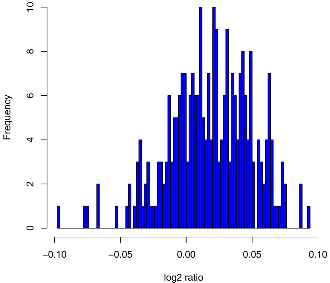
Histogram of log2ratios in 270 HapMap samples at clone Chr4tp-13B11
