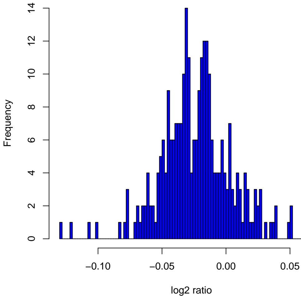
Histogram of log 2 ratios in 270 HapMap samples at clone Chr4tp-13E7
