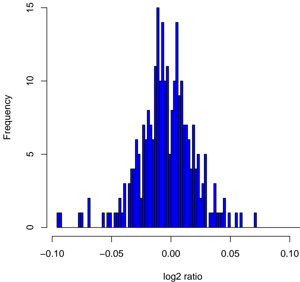
Histogram of log 2 ratios in 270 HapMap samples at clone Chr4tp-13G8
