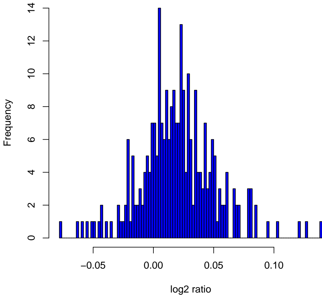
Histogram of log2ratios in 270 HapMap samples at clone Chr4tp-13H12
