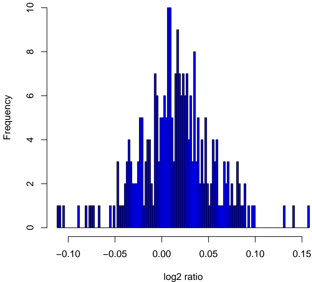
Histogram of log2ratios in 270 HapMap samples at clone Chr4tp-14C3
