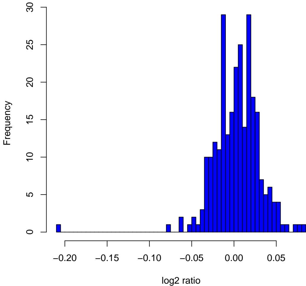
Histogram of log2ratios in 270 HapMap samples at clone Chr4tp-14E10
