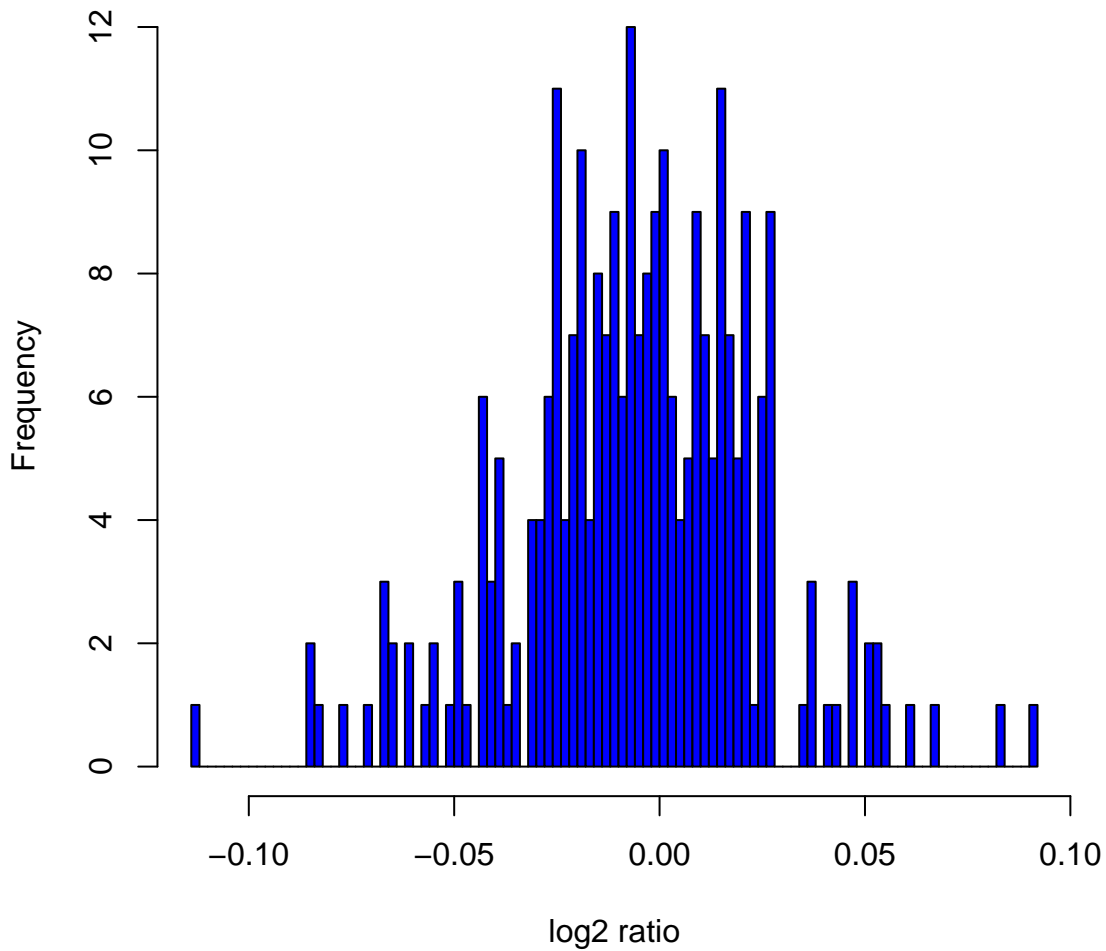
Histogram of log2ratios in 270 HapMap samples at clone Chr4tp-14H7
