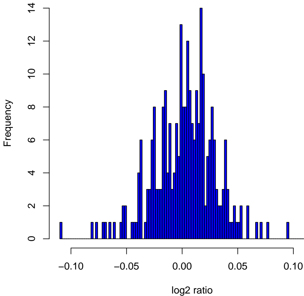
Histogram of log 2 ratios in 270 HapMap samples at clone Chr4tp-14H8
