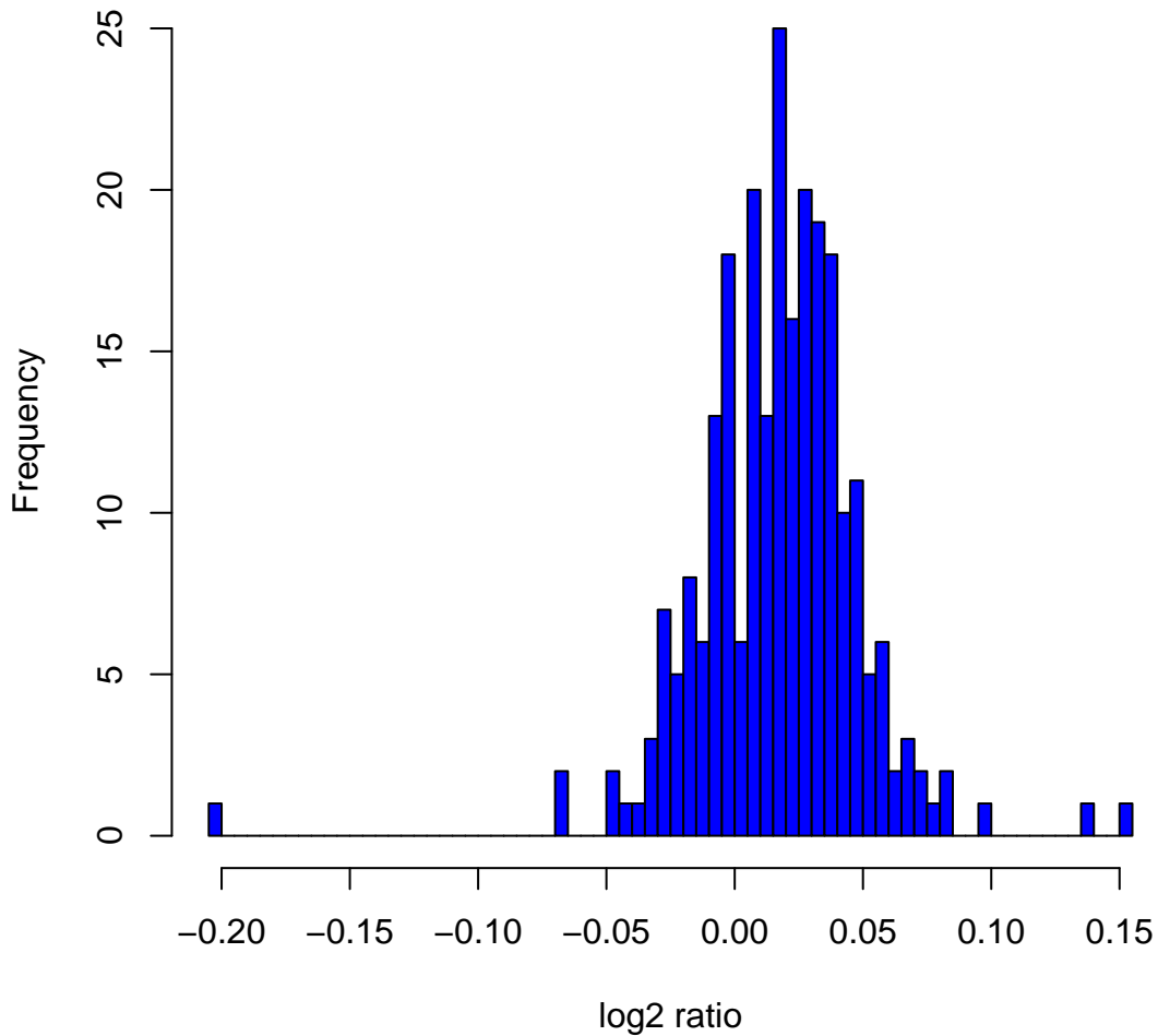
Histogram of log 2 ratios in 270 HapMap samples at clone Chr4tp-15B1
