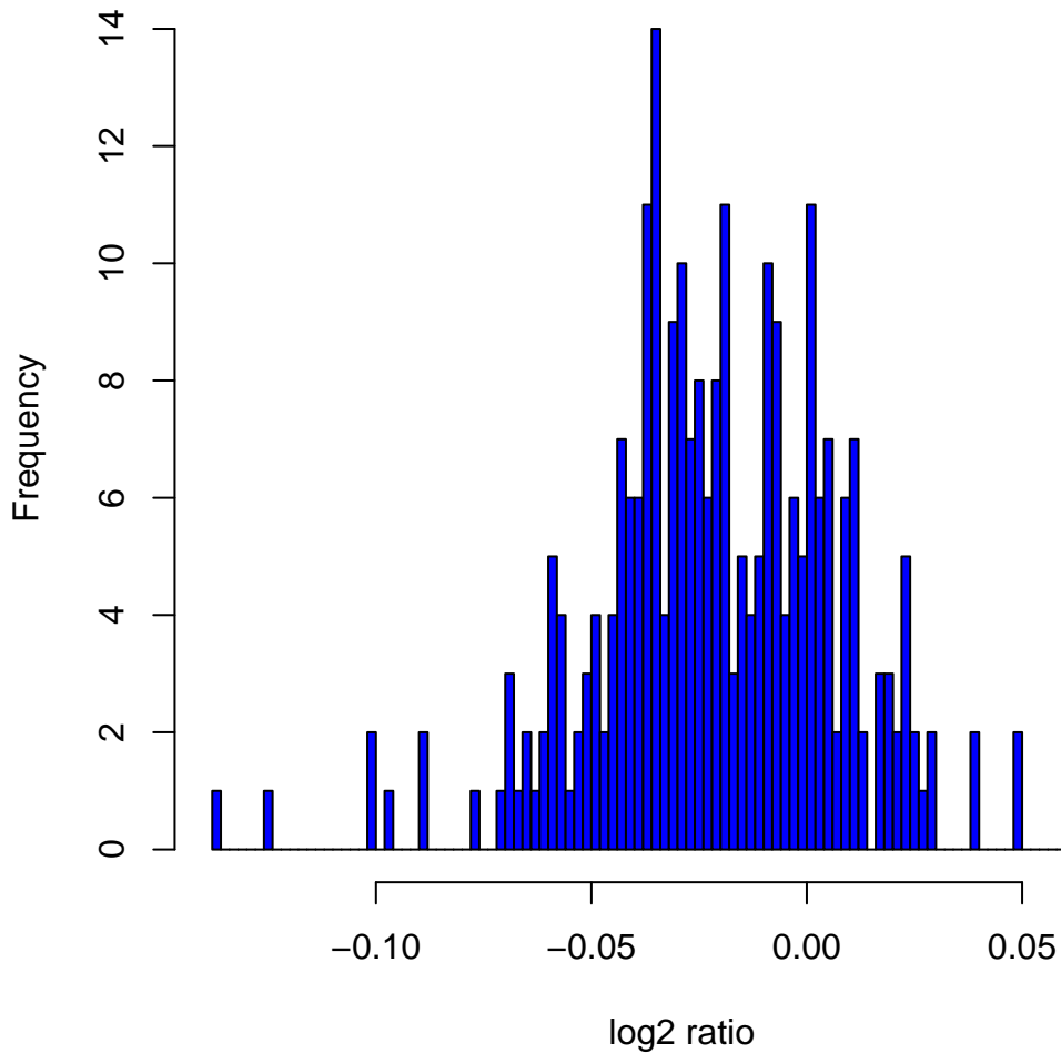
Histogram of log2ratios in 270 HapMap samples at clone Chr4tp-15C10
