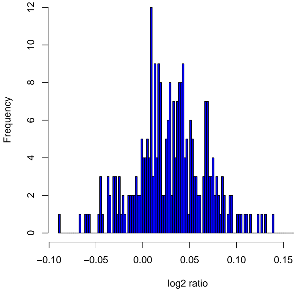
Histogram of log 2 ratios in 270 HapMap samples at clone Chr4tp-15C8
