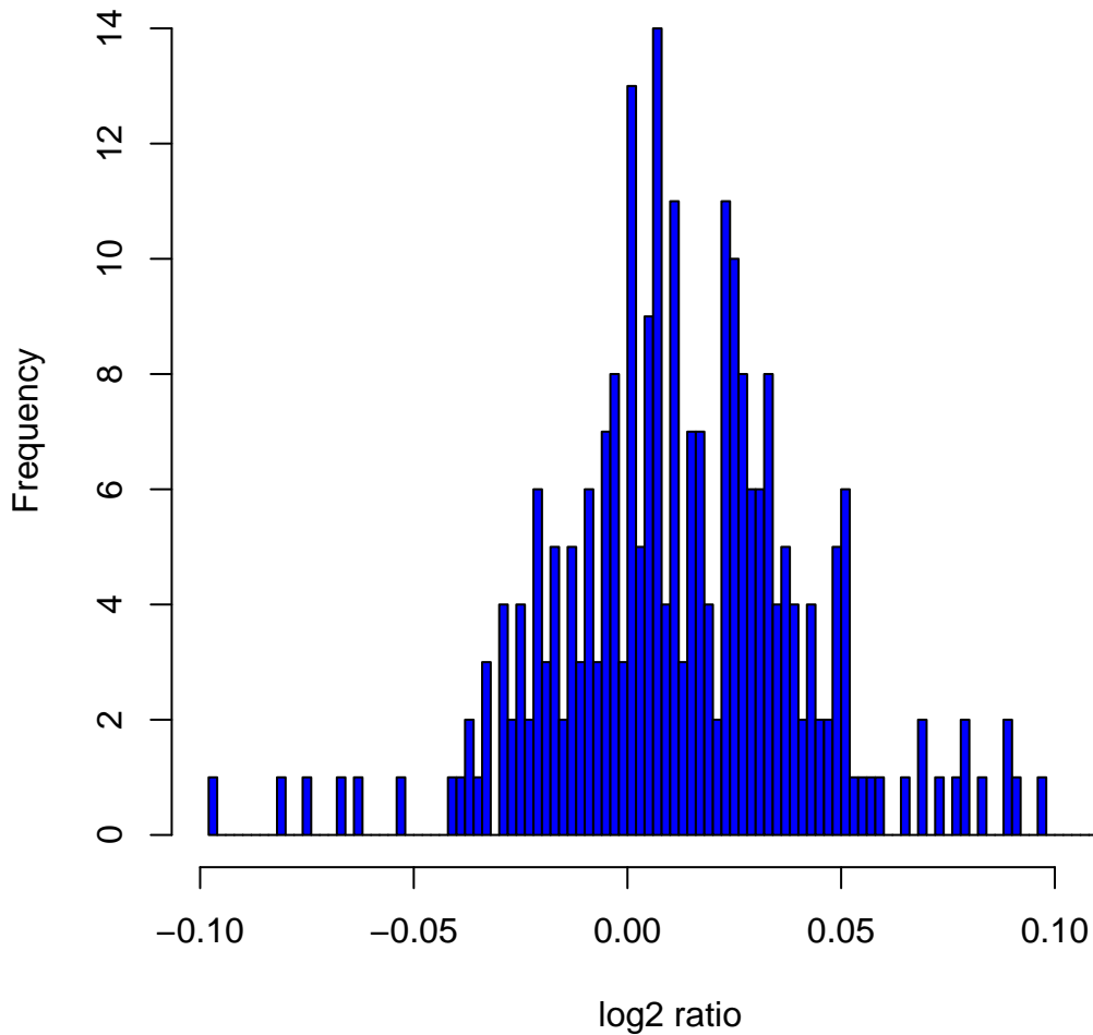
Histogram of \log_2 ratios in 270 HapMap samples at clone Chr4tp-16B1
