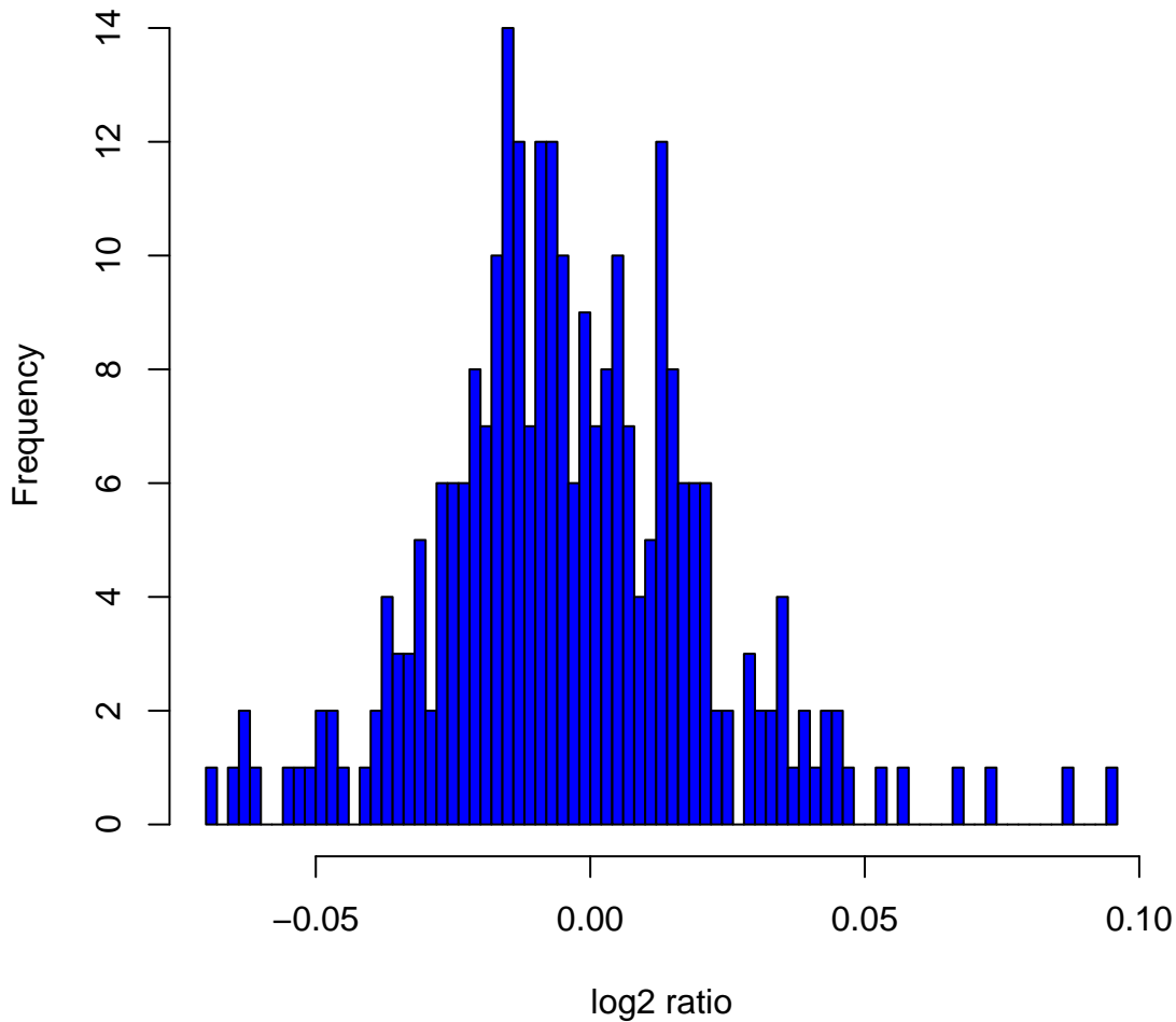
Histogram of log2ratios in 270 HapMap samples at clone Chr4tp-16C10
