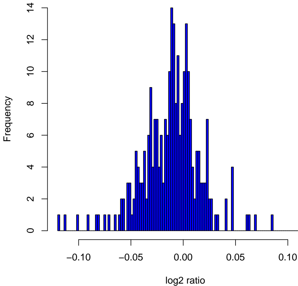
Histogram of log2ratios in 270 HapMap samples at clone Chr4tp-16D10
