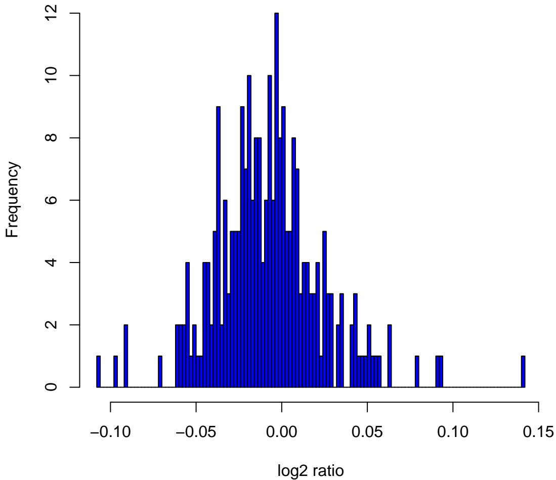
Histogram of \log_2 ratios in 270 HapMap samples at clone Chr4tp-16E5
