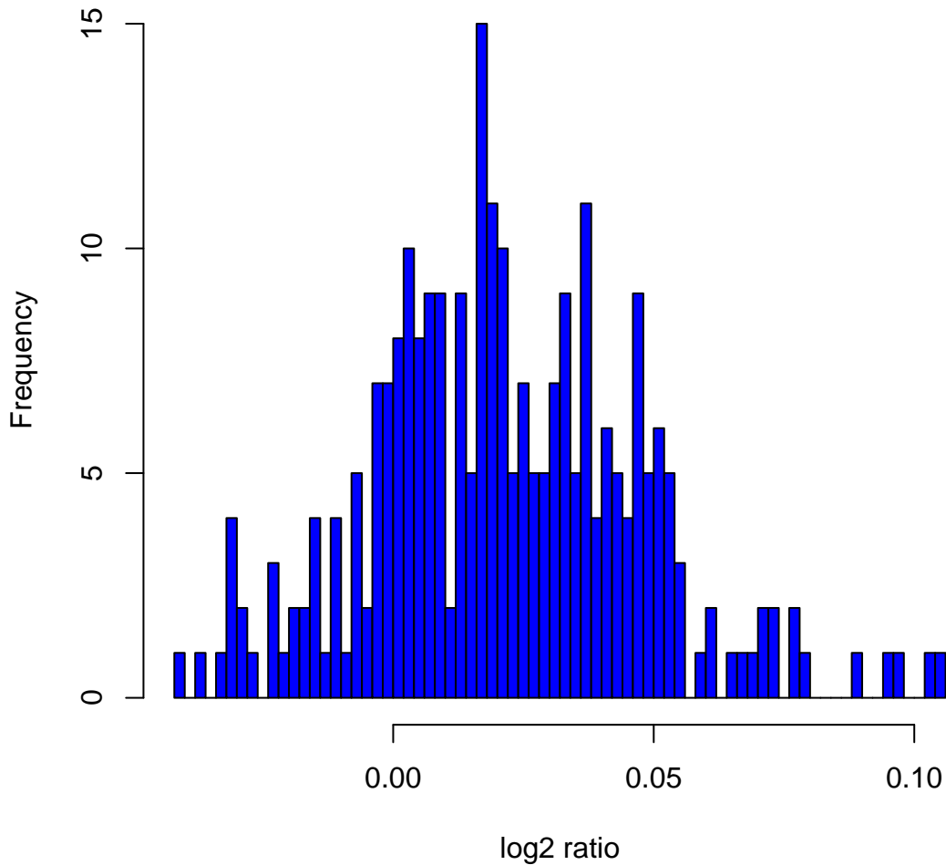
Histogram of log 2 ratios in 270 HapMap samples at clone Chr4tp-16H5
