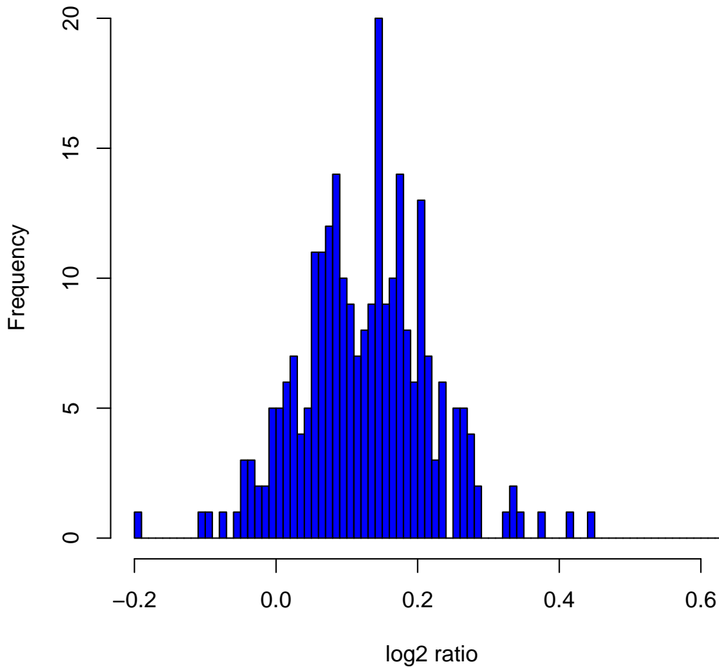
Histogram of log2ratios in 270 HapMap samples at clone Chr4tp-17B12
