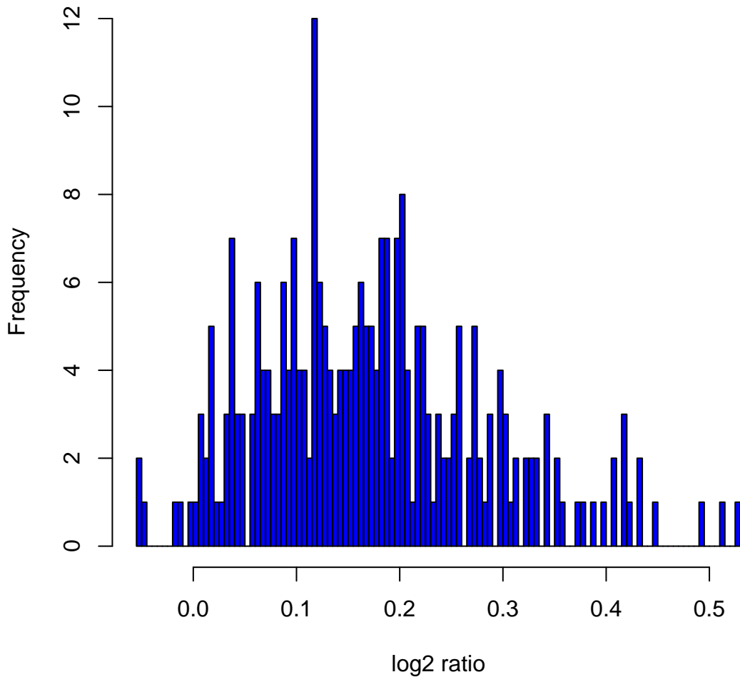
Histogram of log 2 ratios in 270 HapMap samples at clone Chr4tp-17C7
