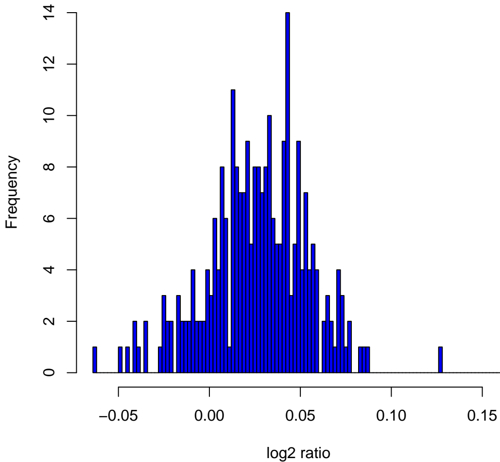
Histogram of \log_2 ratios in 270 HapMap samples at clone Chr4tp-17D1
