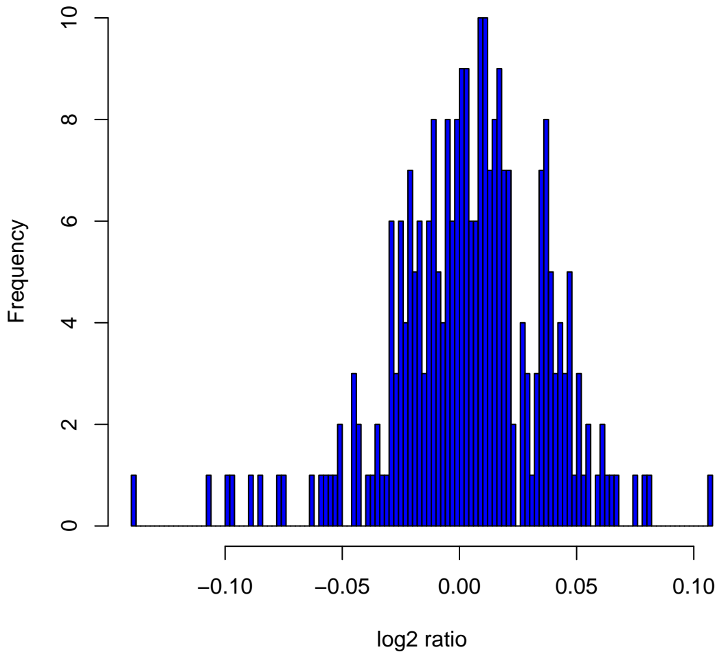
Histogram of log 2 ratios in 270 HapMap samples at clone Chr4tp-17D3
