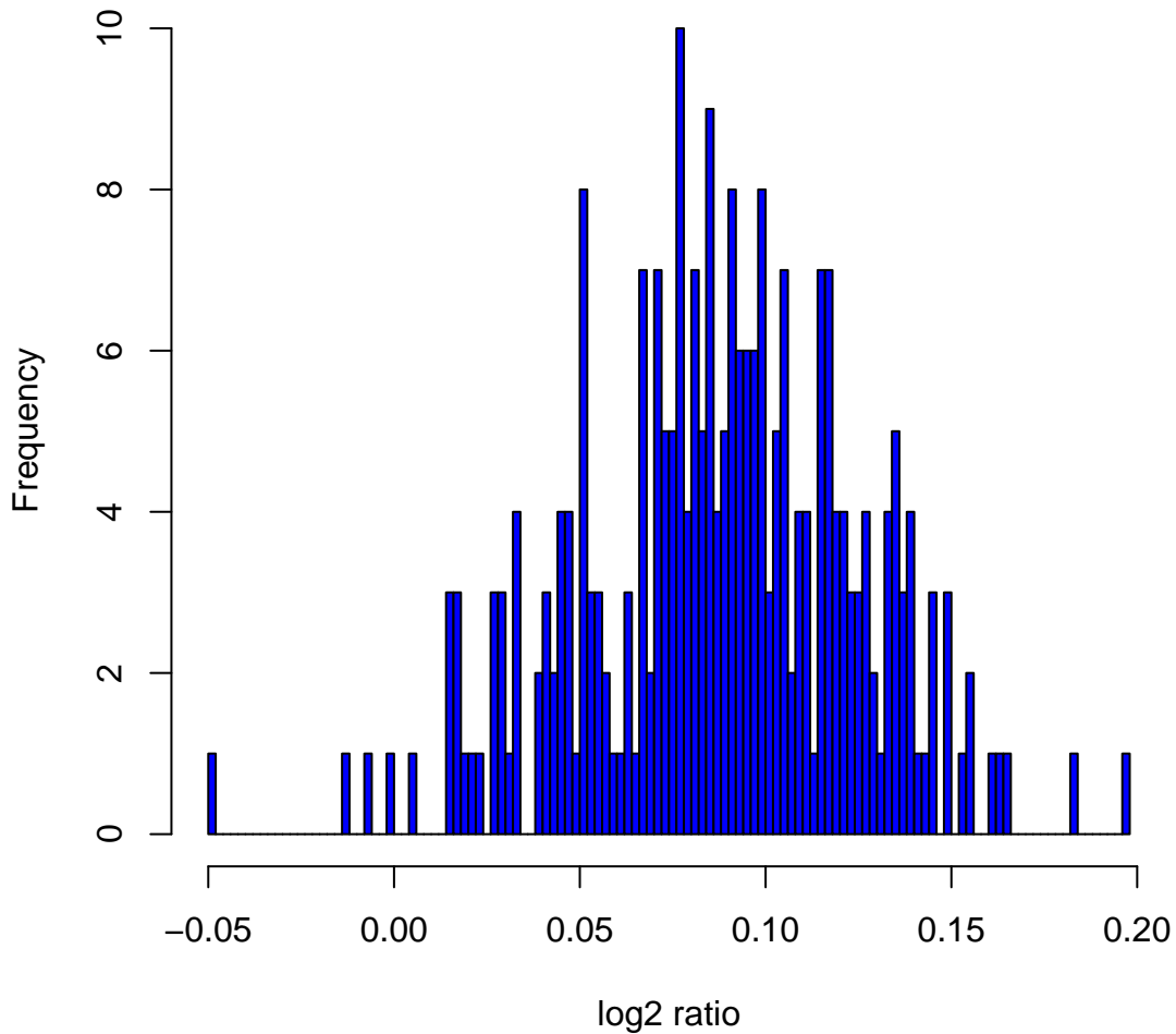
Histogram of log2ratios in 270 HapMap samples at clone Chr4tp-18G11
