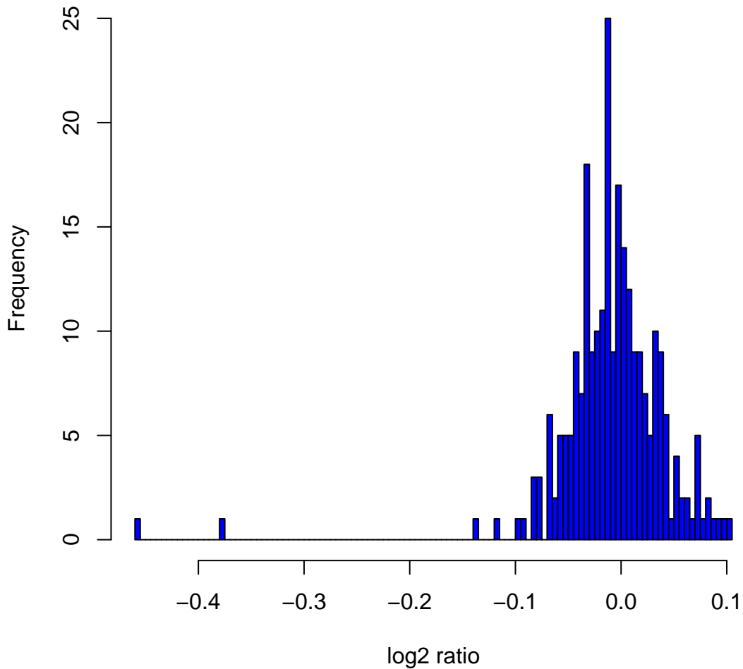
Histogram of log 2 ratios in 270 HapMap samples at clone Chr4tp-18G2
