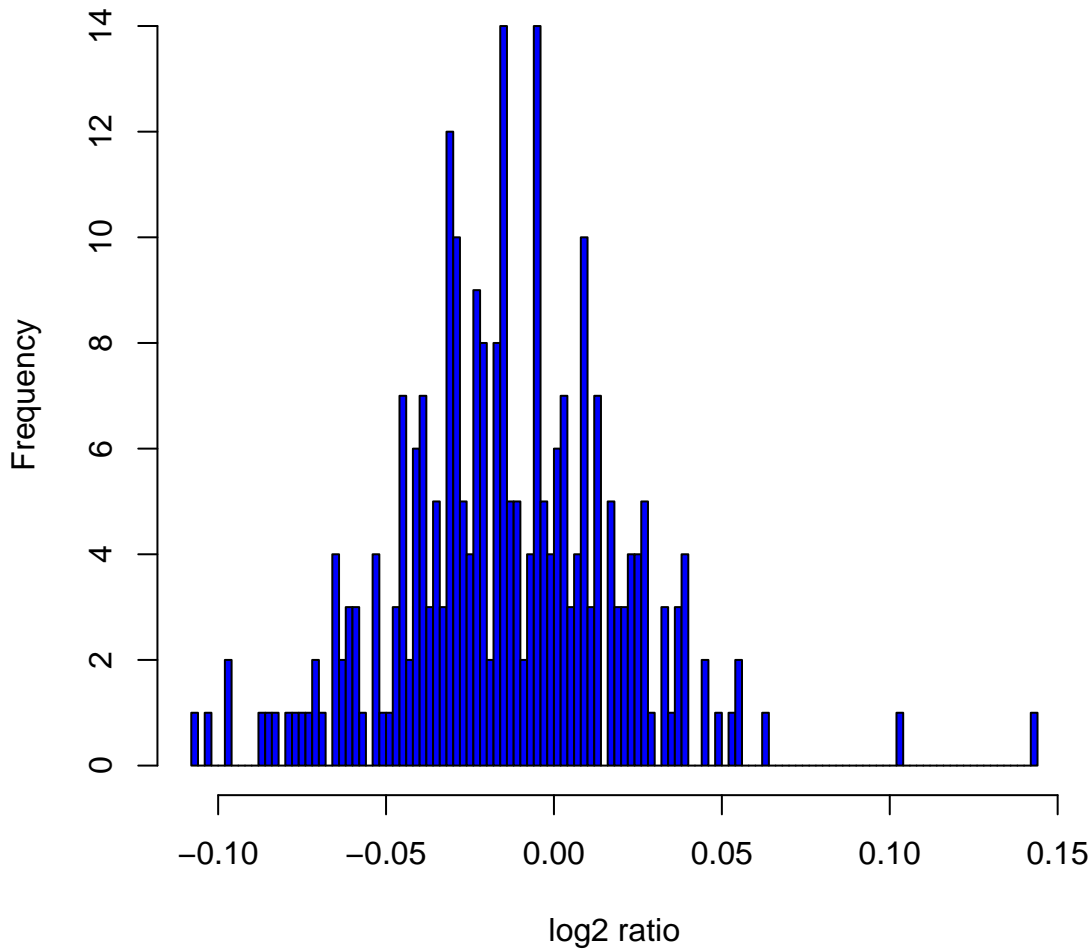
Histogram of log 2 ratios in 270 HapMap samples at clone Chr4tp-1A1
