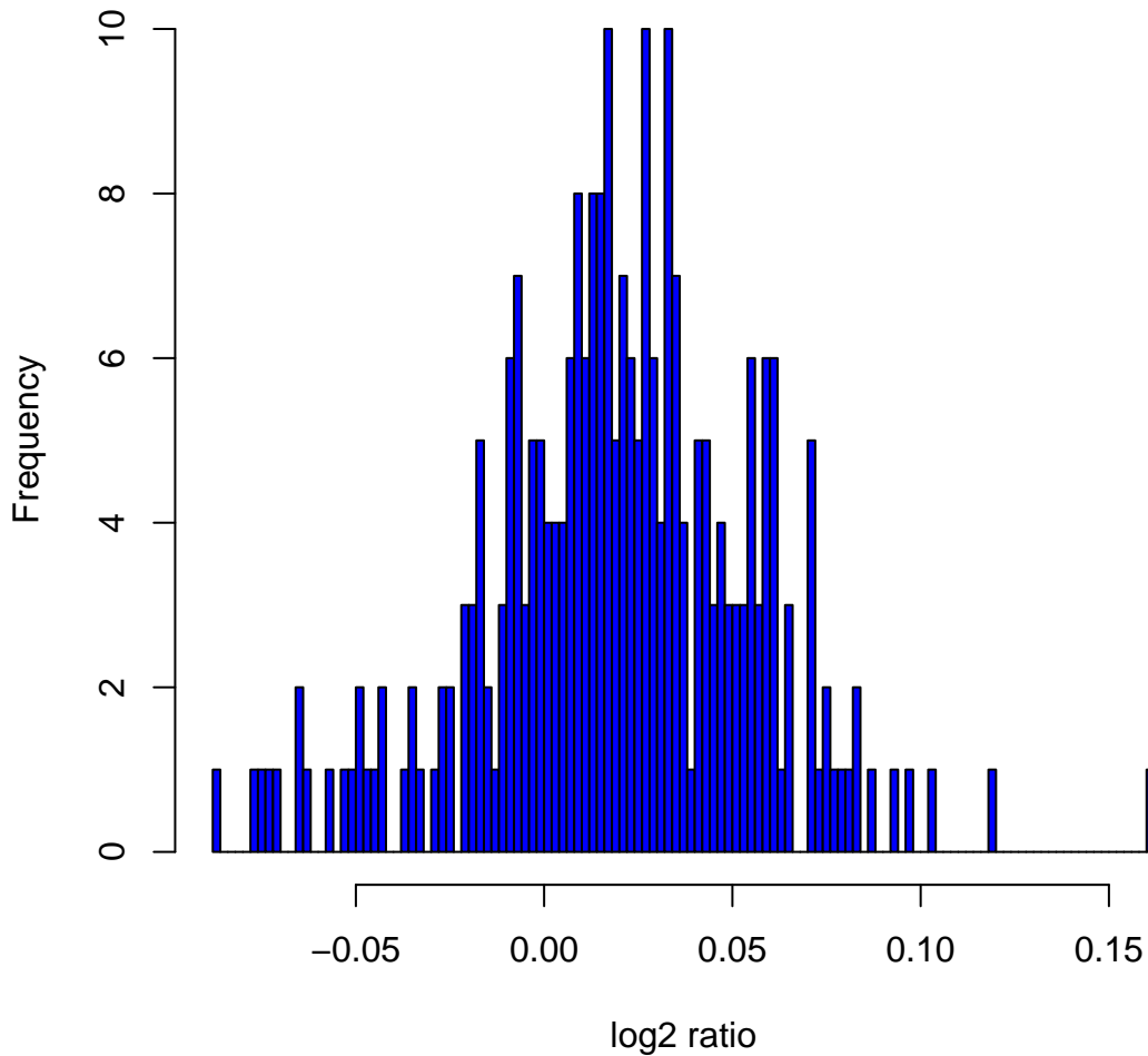
Histogram of log 2 ratios in 270 HapMap samples at clone Chr4tp-1B2
