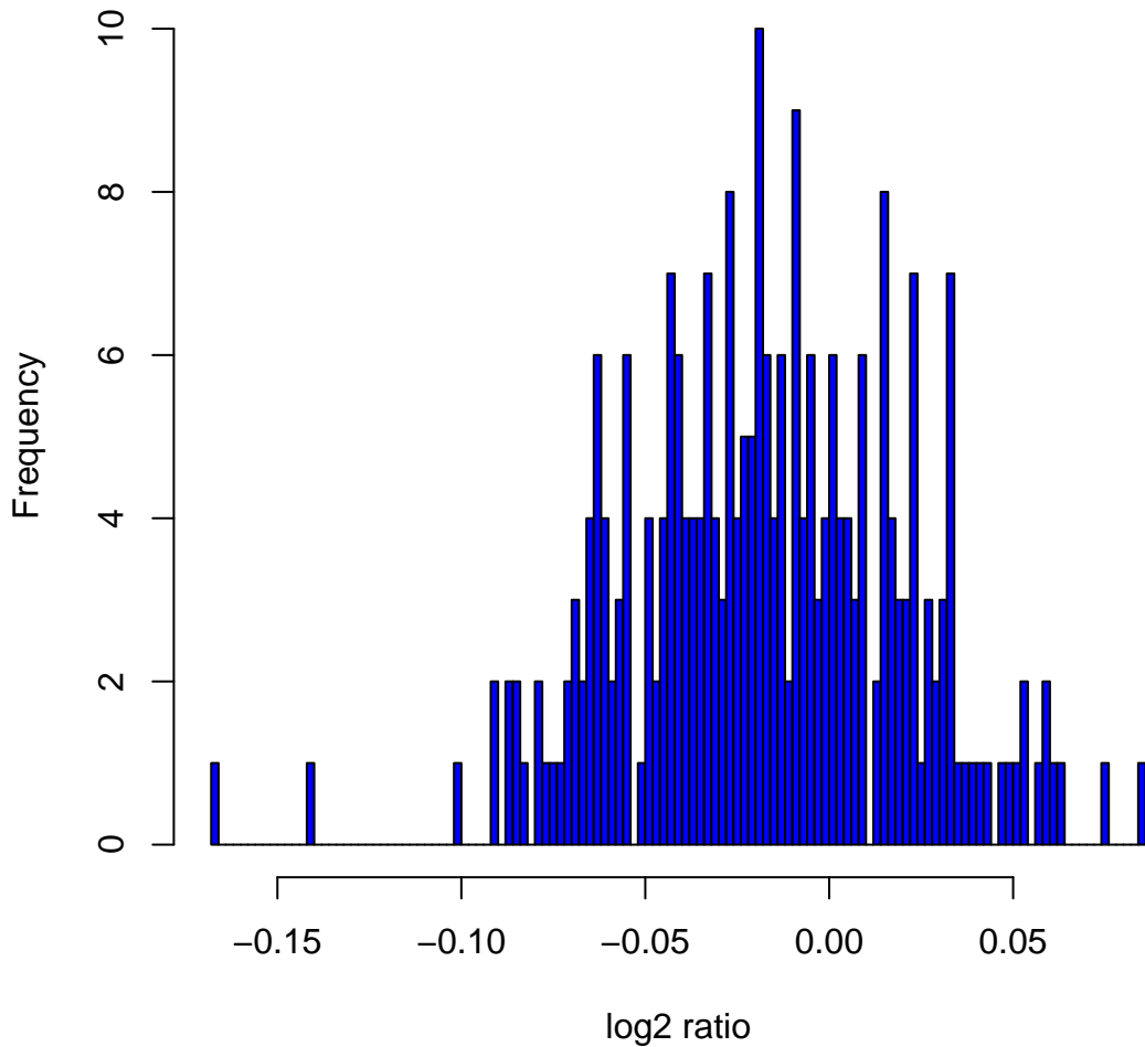
Histogram of log 2 ratios in 270 HapMap samples at clone Chr4tp-1D8
