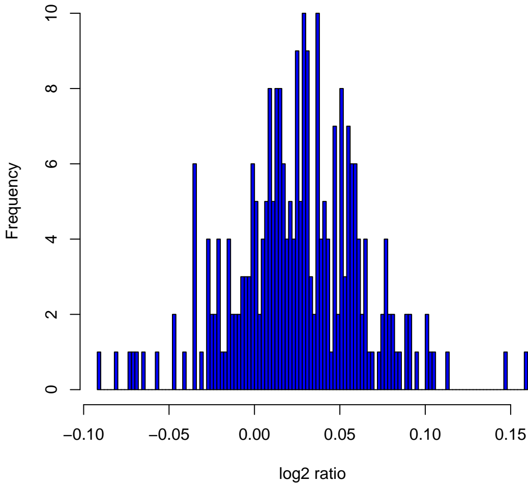
Histogram of log2ratios in 270 HapMap samples at clone Chr4tp-1F8
