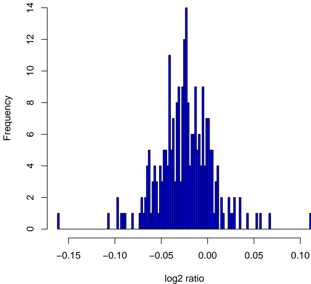
Histogram of log 2 ratios in 270 HapMap samples at clone Chr4tp-1H1
