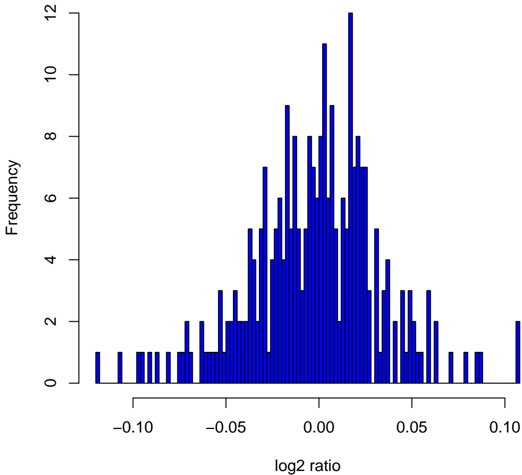
Histogram of log2ratios in 270 HapMap samples at clone Chr4tp-20C10
