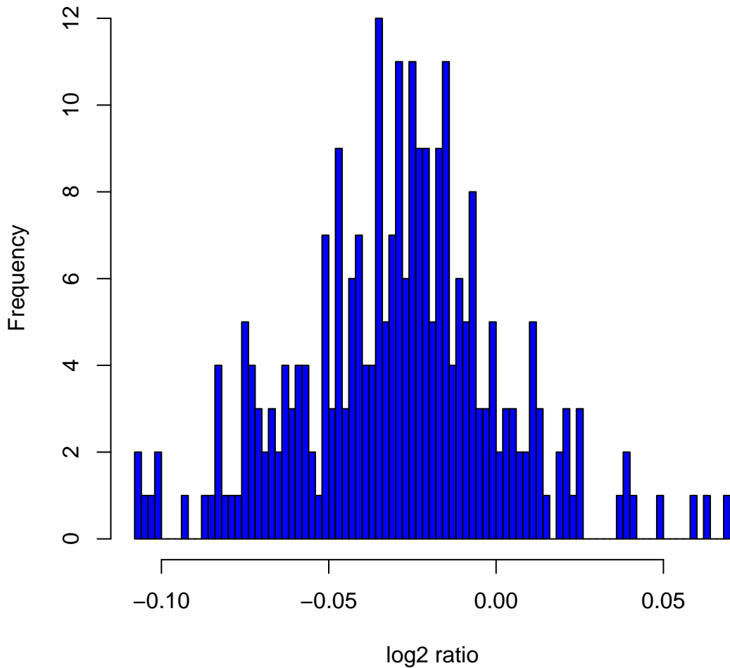
Histogram of log2ratios in 270 HapMap samples at clone Chr4tp-21B12
